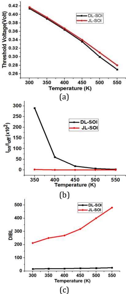
Fig.3 Variation of (a) V_{th} (b) I_{on}/I_{off} (c) DIBL with respect to lattice temperature
