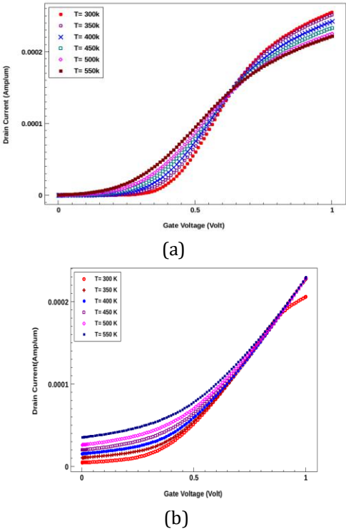
Fig.2 Transfer characteristics of (a) DL-SOI (b) JL-SOI with respect to lattice temperature
