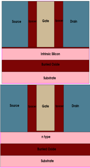
Fig.1 (a) DL SOI Structure (b) JL SOI Structure
